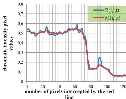
Fig. 12. Comparison between pixel intensity profiles
