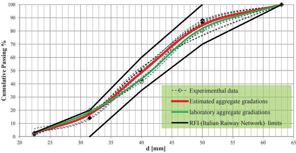
Fig. 17. Granulometric curve, Position No. 1
