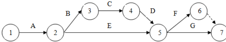
Diagram 1. The sequence of steps in the adopted technology. A - execution of the floor covering, B - preparation of landings, C – laying the terrazzo flooring on landings, D - installation of plinths on landings, E - installation of stair plinths, F –grouting, G - silicone sealing.
