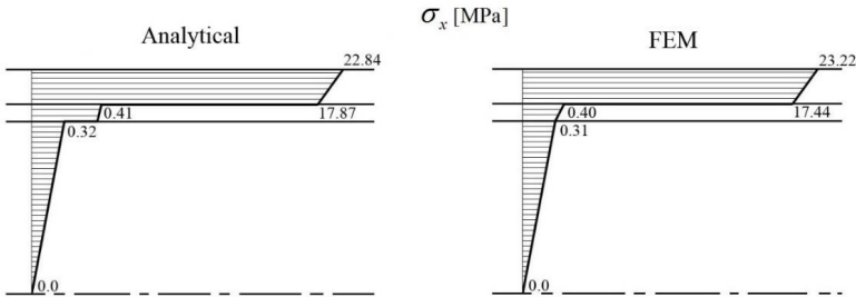
Fig 5. Normal stresses
