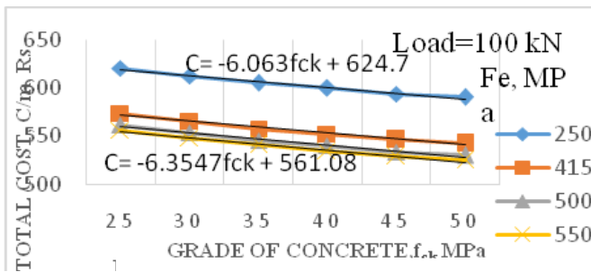
Fig. 8. Variation of Total Cost with grades of Steel and Concrete.
