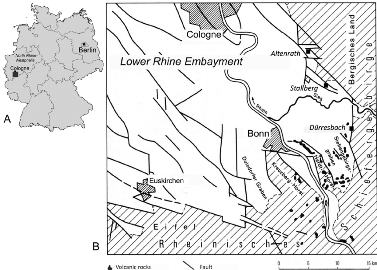
Fig. 1. Location of the investigated area in Germany (A), and the sites at the south-eastern border of the Lower Rhine Embayment (B, modified after Burghardt 1979)
