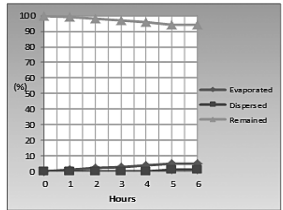
Fig. 7d. (S:4). Fuel Oil degradation chart
