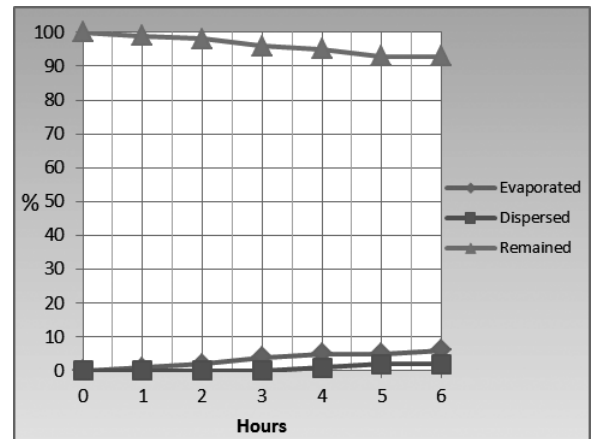
Fig. 7b. (S:2). Fuel Oil degradation chart
