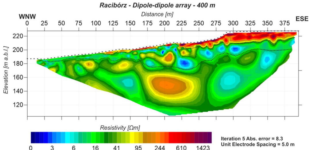
Fig.8. Resistivity model of ERT profile carried out on the Racibórz landslide in 2016. Dipole-dipole array. Dotted line: boundary of resistivity complex.
