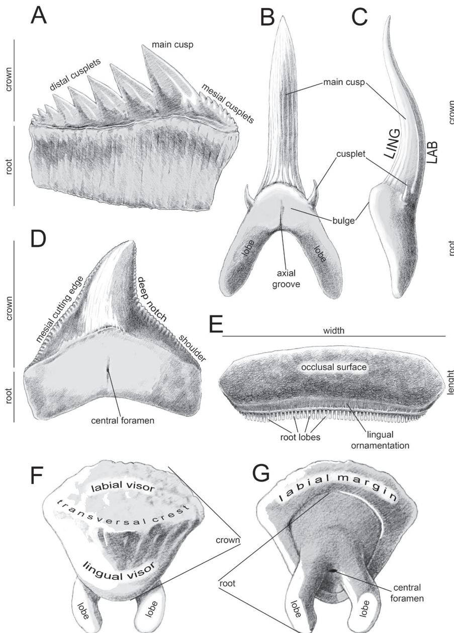
Fig. 5. Tooth terminology of the chondrichthyan remains. A — Hexanchidae tooth in lingual view. B — Odontaspidae tooth in lingual view; C — in mesiodistal view (lab: labial side, lin: lingual side). D — Carcharhinidae tooth in lingual view. E — Myliobatidae tooth in semi-occlusal/lingual view. F — Dasyatidae tooth in occlusal; G — in basal view (after Cappetta 2012).
