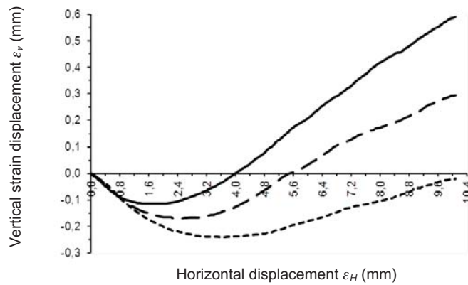
Fig. 3. Deformation curves obtained for corn using the square shear cell. Explanations as in Fig. 1.
