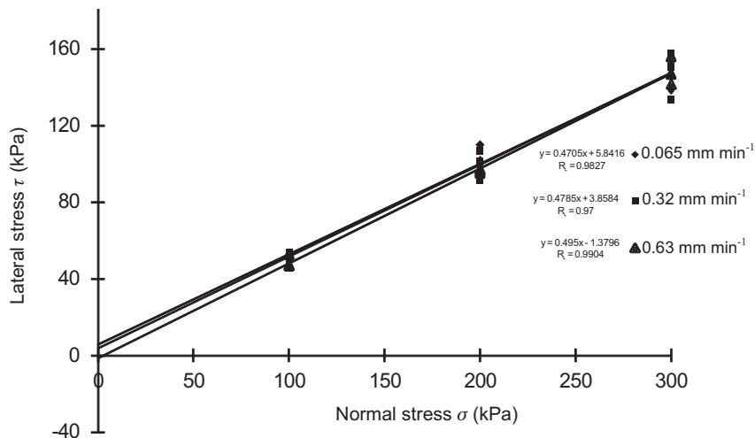
Fig. 2. Mohr-Coulomb strength envelopes obtained for corn using the square shear cell.
