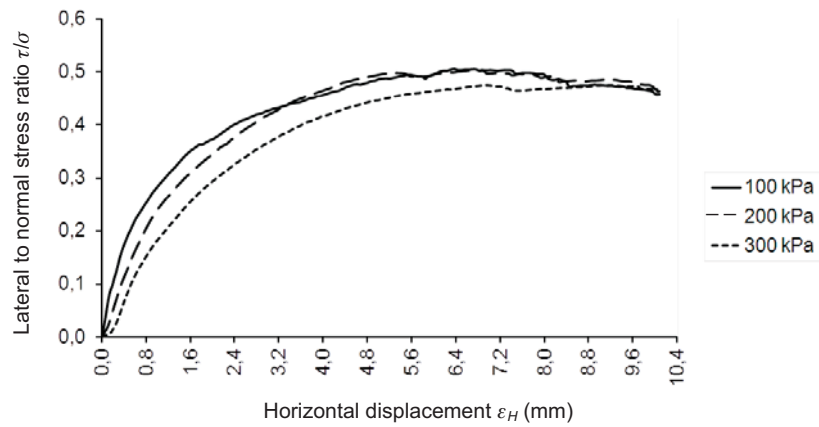
Fig. 1. Stress-strain curves obtained for corn tested at 0.065 \text{ mm min}^{-1} using the square shear cell.
