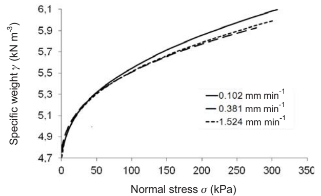
Fig. 5. Variation of the specific weight with normal pressure. 'Prevision' oats.
