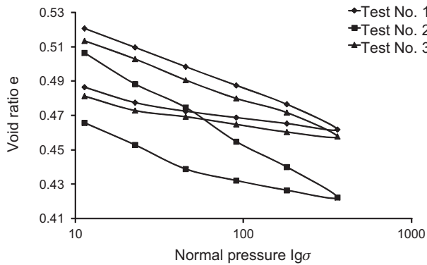
Fig. 4. Oedometer curves obtained for lentil vetch.
