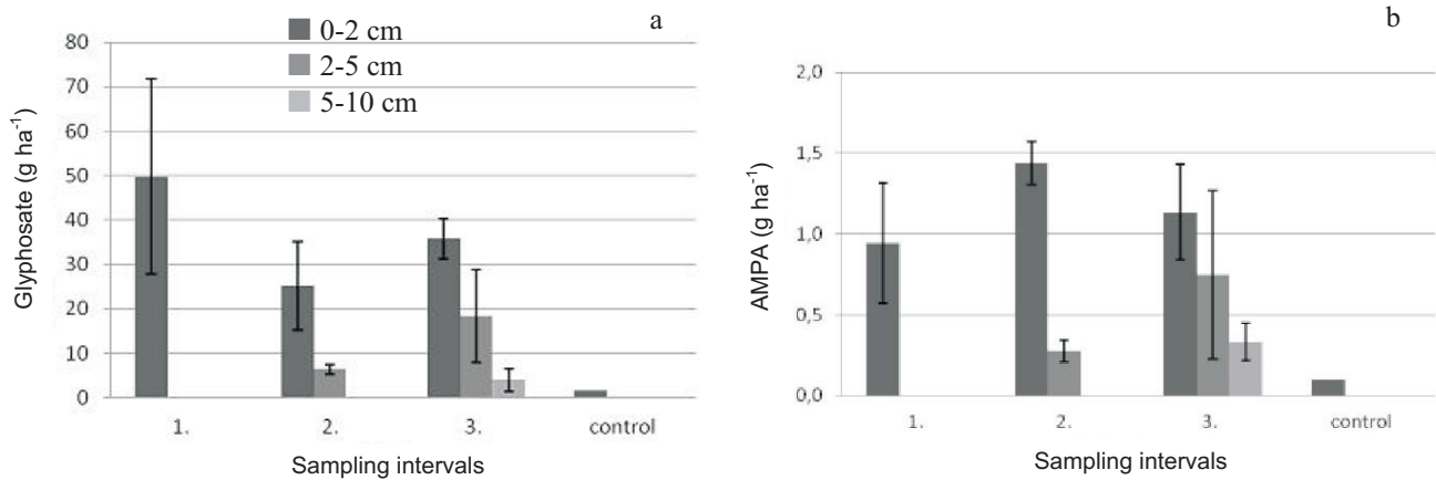
Fig.1. Content of: a – glyphosate and b – AMPA in Chernozem at different time intervals and soil depths, sampling: 1. – immediately after application, 2. – 3 days after application, 3. – 10 days after application; control – residues before application.
