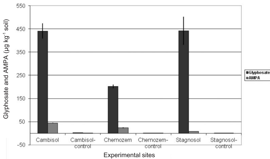
Fig. 4. Glyphosate and AMPA contents in the investigated soils at 0-2 cm soil depth. The control values show the glyphosate contents before application (eg the residual traces, next to zero, from the previous application).
