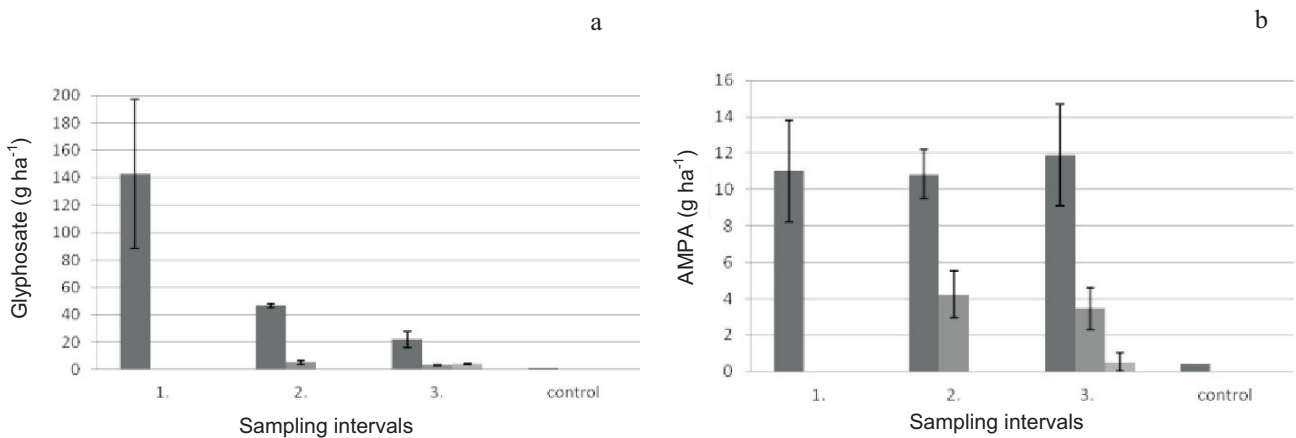
Fig. 3. Content of: a – glyphosate and b – AMP contents in Cambisol at different time intervals and soil depths, sampling: 1. – immediately after application, 2. – 3 days after application, 3. – 12 days after application; control – residues before application.
