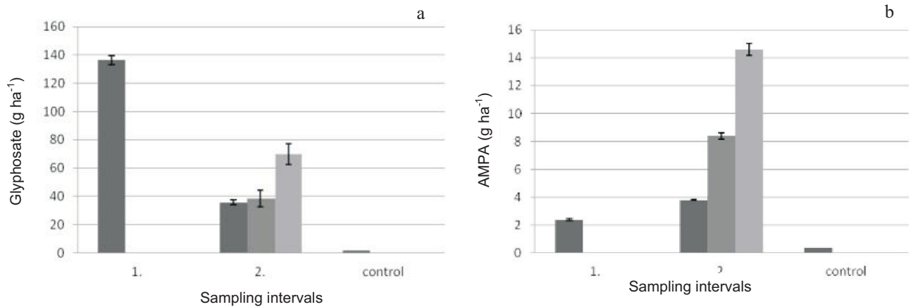
Fig. 2. Content of: a – glyphosate and b – AMPA in Stagnosol at different time intervals and soil depths, sampling: 1. – immediately after application, 2. – 28 days after application; control – residues before application.
