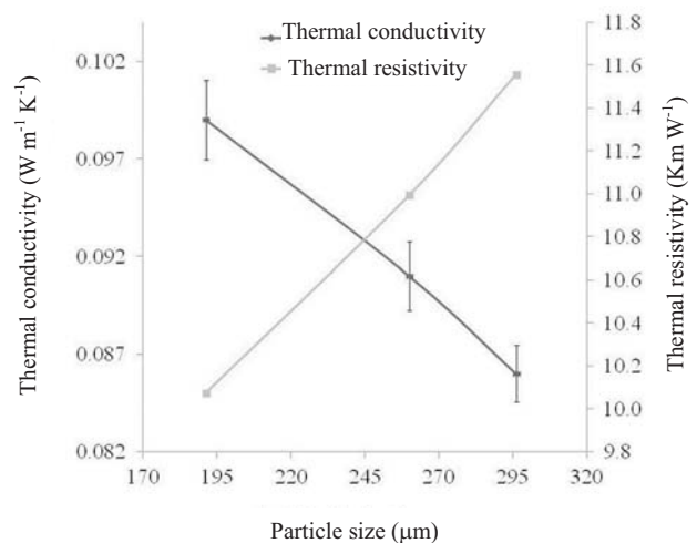
Fig. 1. Effect of particle size on thermal properties of mango pulp powder.
