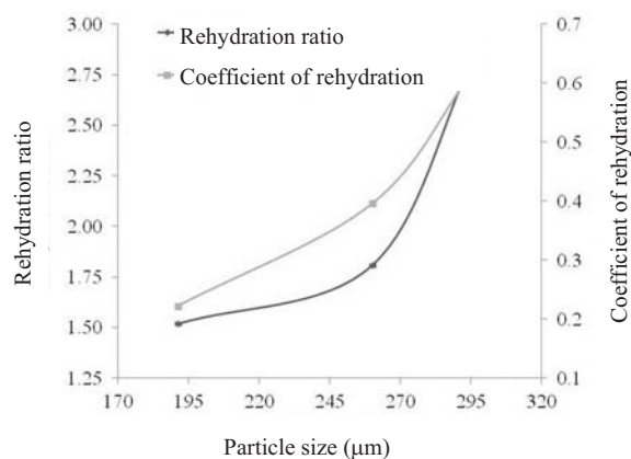
Fig. 2. Effect of particle size on the rehydration ratio and the coefficient of rehydration of mango pulp powder.
