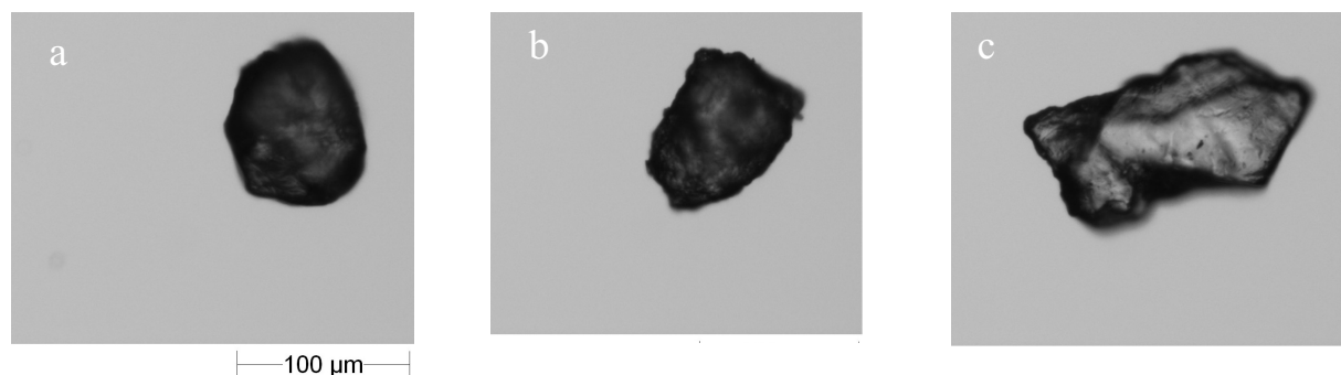
Fig. 1. Characteristic shapes of the sand grains from the three investigated sediments: a – Pieszowola, b – Pierwoszków, and c – Murowaniec.
