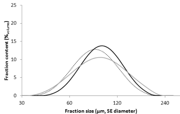
Fig. 4. PSDs of the investigated sand samples obtained by the LDM. Explanations as in Fig. 2.
