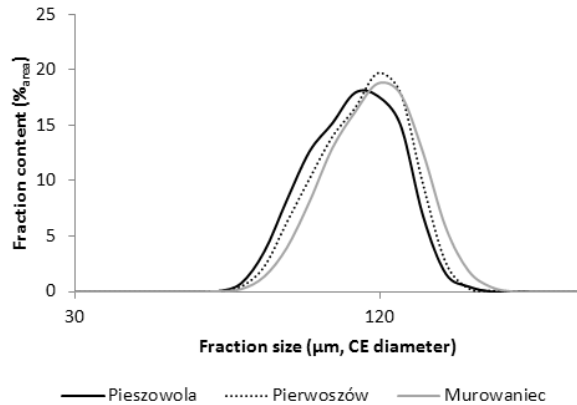
Fig. 2. PSDs (expressed as the CE diameter) of the investigated sands obtained by the image analysis from the optical microscope.
