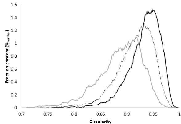
Fig. 3. Distribution of circularity of the investigated sands obtained by the image analysis from the optical microscope. Explanations as in Fig. 2.
