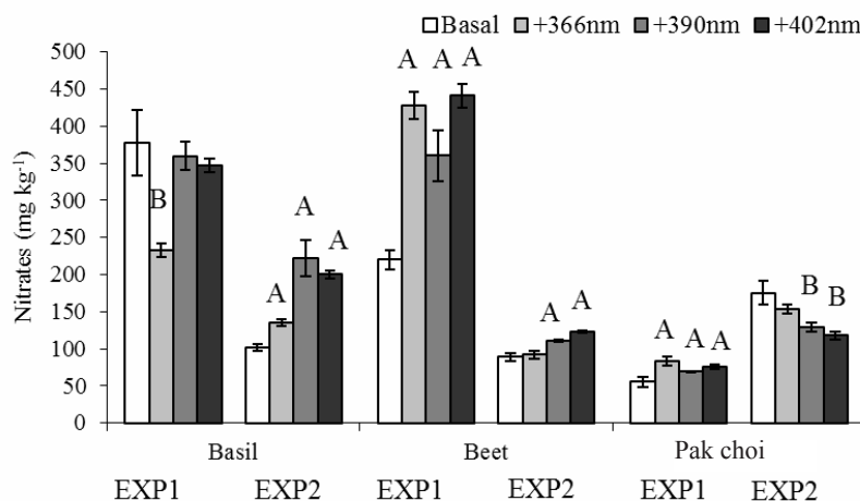
Fig. 3. Effect of UV-A on the nitrate content in the microgreens: A – significantly higher than the control (basal illumination), B – significantly lower than the control. Significance level: p < 0.05 (t-test).
