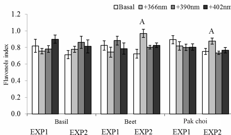
Fig. 2. The effect of UV-A on the flavonol index of the microgreens: A – significantly higher than the control (basal illumination), Significance level: p < 0.05 (t-test).
