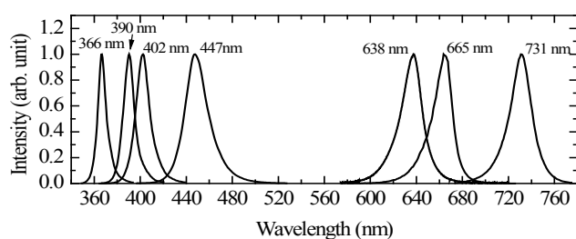
Fig. 1. Normalized emission spectra of the LEDs used in the lighting equipment.
