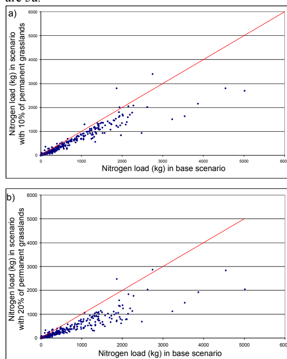
Fig. 5. Changes in nitrate nitrogen load in the Zgłowiączka River catchment for the scenarios of permanent grassland share in the catchment: a) 10%, b) 20%; source: own study
