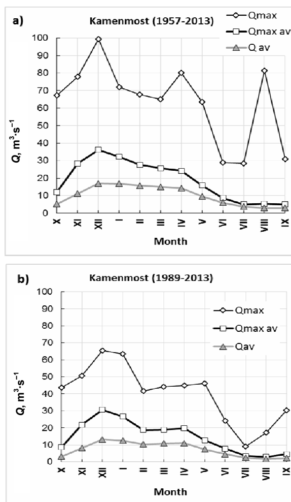
Fig. 3. Characteristic monthly discharges in Kamenmost: a) in the operation period, b) after Ricice reservoir; Q_{\max} = maximum recorded discharge, Q_{\max \text{ av}} = mean maximum monthly discharge, Q_{\text{av}} = mean monthly discharge; source: own study
