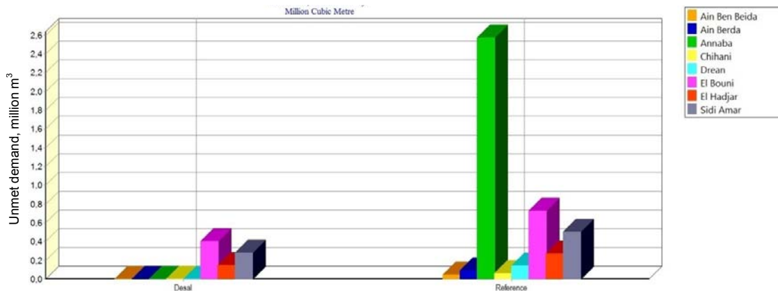
Fig. 9. Comparison of unmet demand of both scenarios Reference and seawater Desalination (Desal) – January 2030; source: own study
