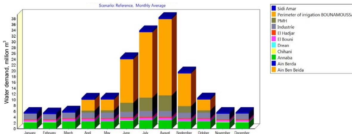
Fig. 3. Monthly water demand – scenario Reference; source: own study
