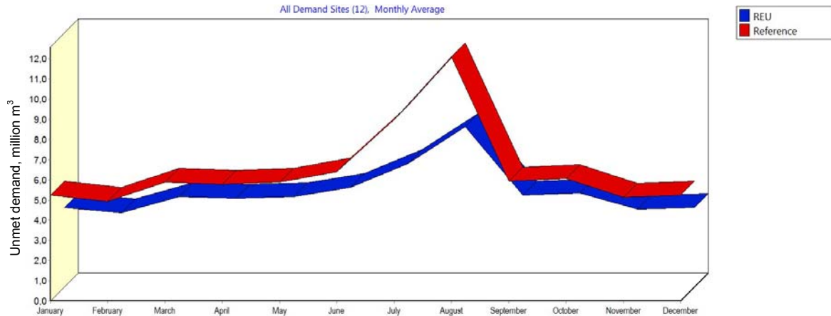
Fig. 7. Unmet demand of the two scenarios Reference and Water Reuse (REU); source: own study
