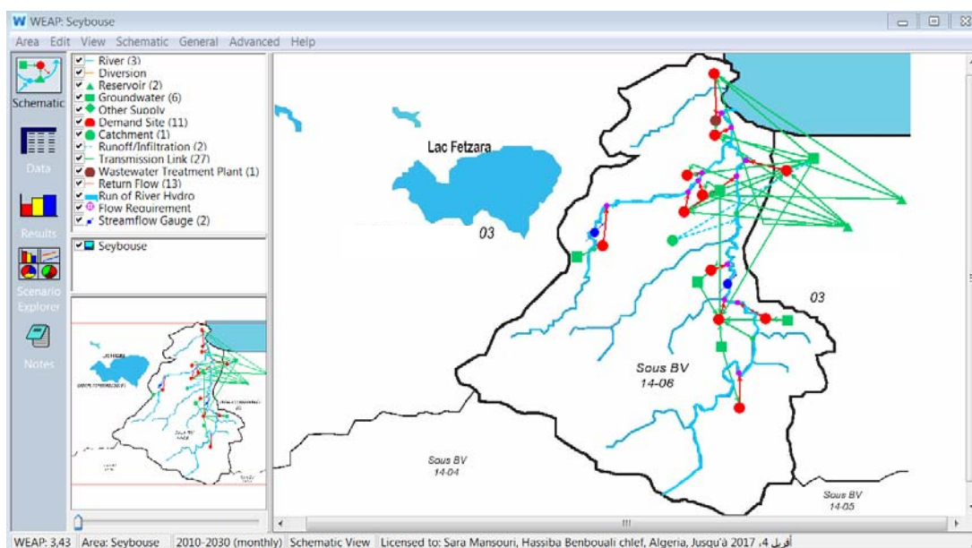
Fig. 2. Final map presentation of watershed by Evaluation and Water Planning (WEAP) model; source: own elaboration
