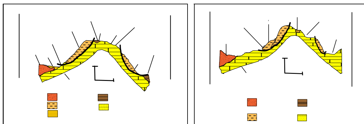
Fig. 11. Geological sections; source: FOURCADE, RAOULT [1973]
