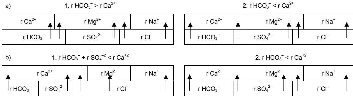
Fig. 10. Representation of the dissolved salts of the Hammam Maskoutaine's thermo-mineral waters: a) low water, b) high water; r = atomic mass/equivalent ( \text{meq}\cdot\text{dm}^{-3} ); source: own study
