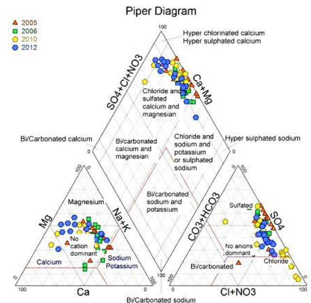
Fig. 6. Piper diagram; source: own study
