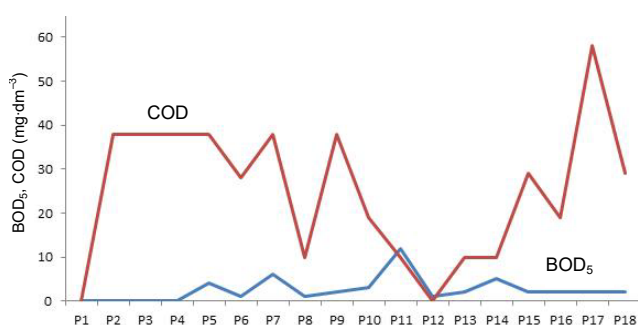
Fig. 9. Variation of BOD 5 and COD in the M'zab valley; P1–P18 = measurement points as in Fig. 3; source: own study
