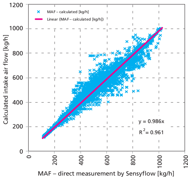
FIGURE 1: Comparison of calculated mass air flow with mass air flow derived from a laboratory-grade mass air flow meter on Iveco Tector heavy-duty on-road diesel engine.
