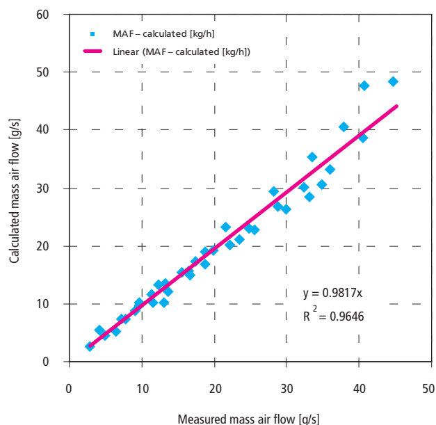
FIGURE 5: Comparison of calculated mass air flow with mass air flow computed from orifice measurement on a Škoda Fabia 1.2 HTP gasoline engine.
