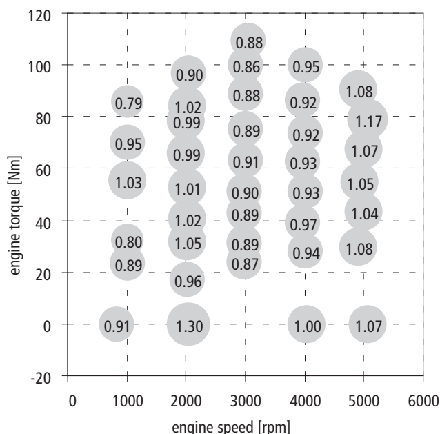
FIGURE 7: Ratio of calculated to measured mass air flow at different engine speed and loads on a Škoda Fabia 1.2 HTP gasoline engine.
