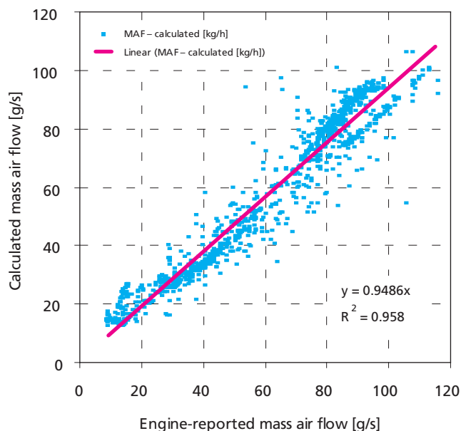
FIGURE 3: Comparison of calculated mass air flow with mass air flow derived from an on-board mass air flow sensor on a Renault Traffic turbodiesel engine during freeway operation.
