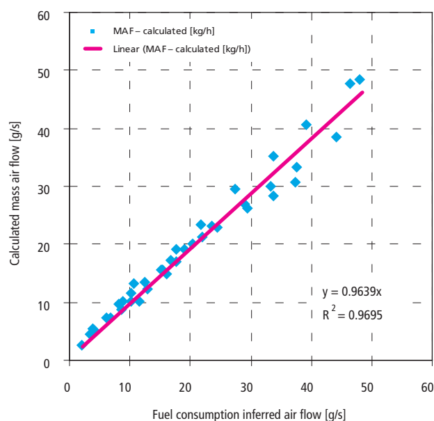
FIGURE 6: Comparison of calculated mass air flow with mass air flow computed from measured fuel consumption and air-fuel ratio computed from exhaust composition on a Škoda Fabia 1.2 HTP gasoline engine.
