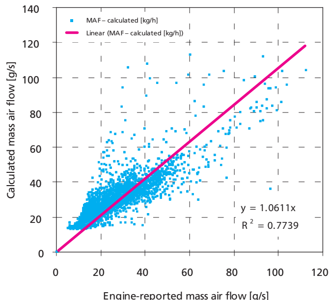
FIGURE 4: Comparison of calculated mass air flow with mass air flow derived from an on-board mass air flow sensor on a Renault Traffic turbodiesel engine during city and highway driving.
