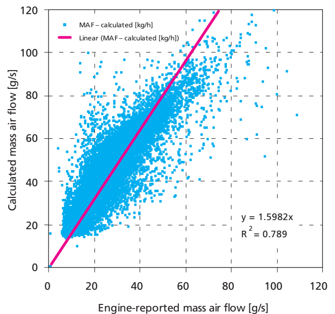
FIGURE 2: Comparison of calculated mass air flow with mass air flow reported by the ECU on a Škoda Octavia 2.0 TDI diesel engine.
