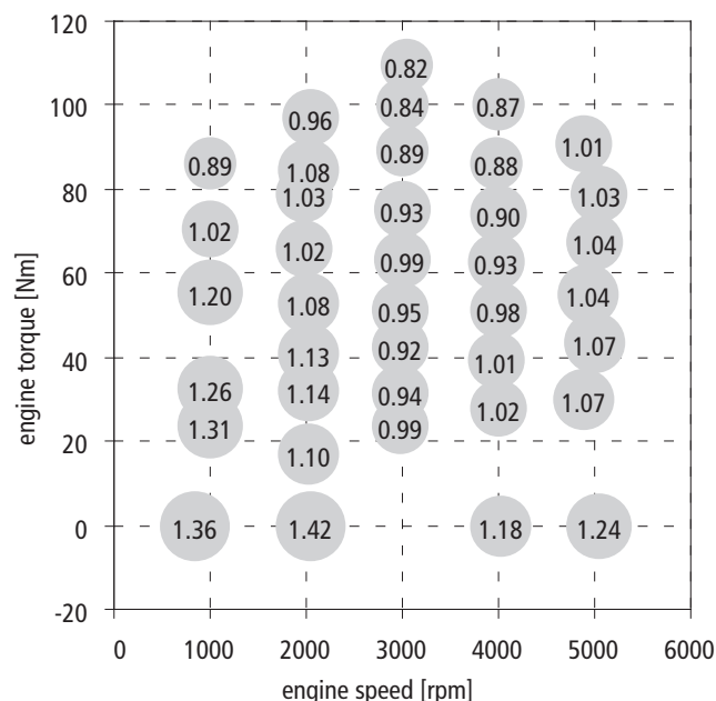
FIGURE 8: Ratio of calculated to fuel-consumption-derived mass air flow at different engine speed and loads on a Škoda Fabia 1.2 HTP gasoline engine.
