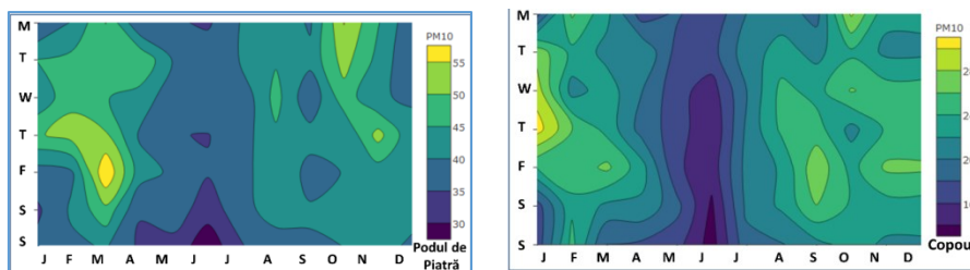
Fig. 6. Weekly cycle at annual level of mean daily concentrations in air quality monitoring points of metropolitan region of Iași (2013-2015)
