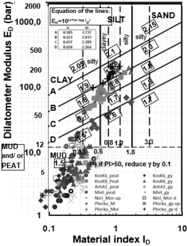
FIGURE 4. Chart for estimating soil type and unit weight – normalized to \gamma_w (Marchetti and Crapps 1981)
